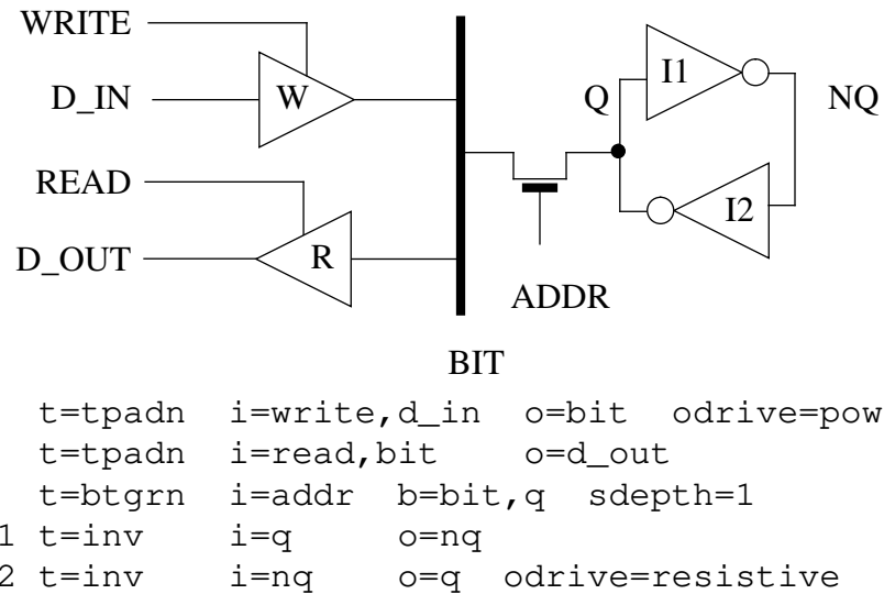
Figure 2.7-9 Memory Cell Read/Write Circuit
